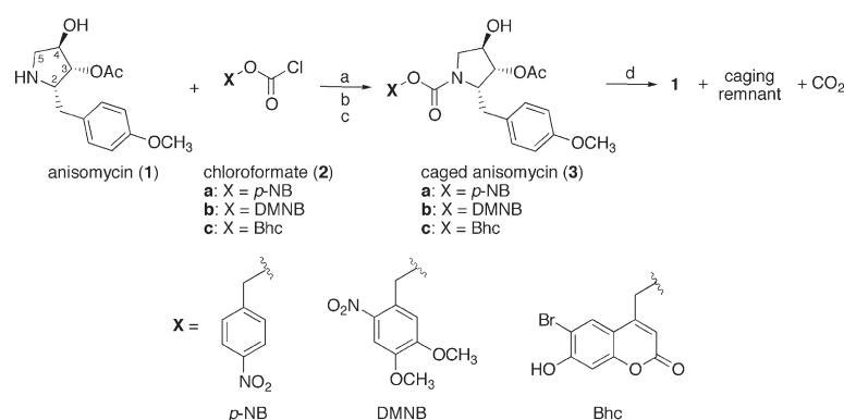
Figure 1. Synthesis and Photochemical Reaction of Caged Anisomycins
